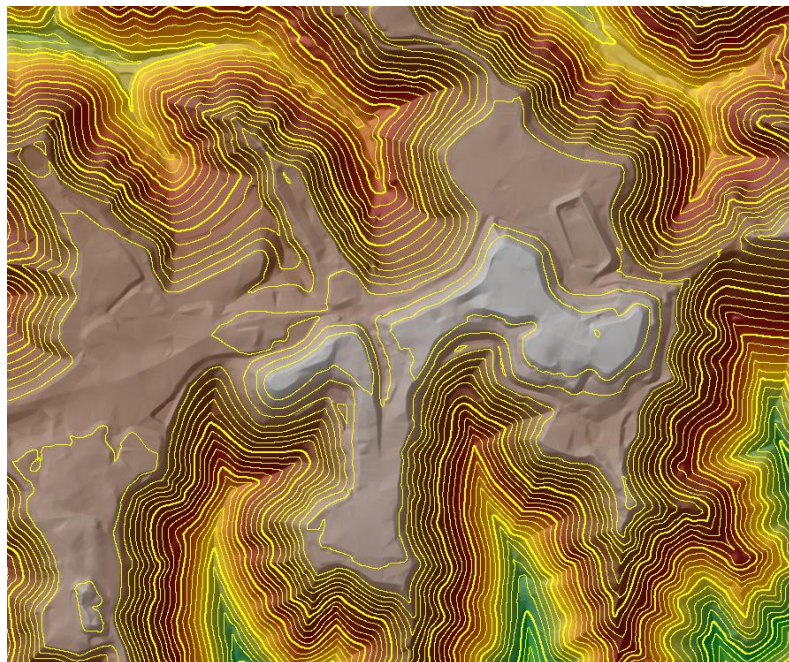
Figure 4. Forty foot contours and DTM
