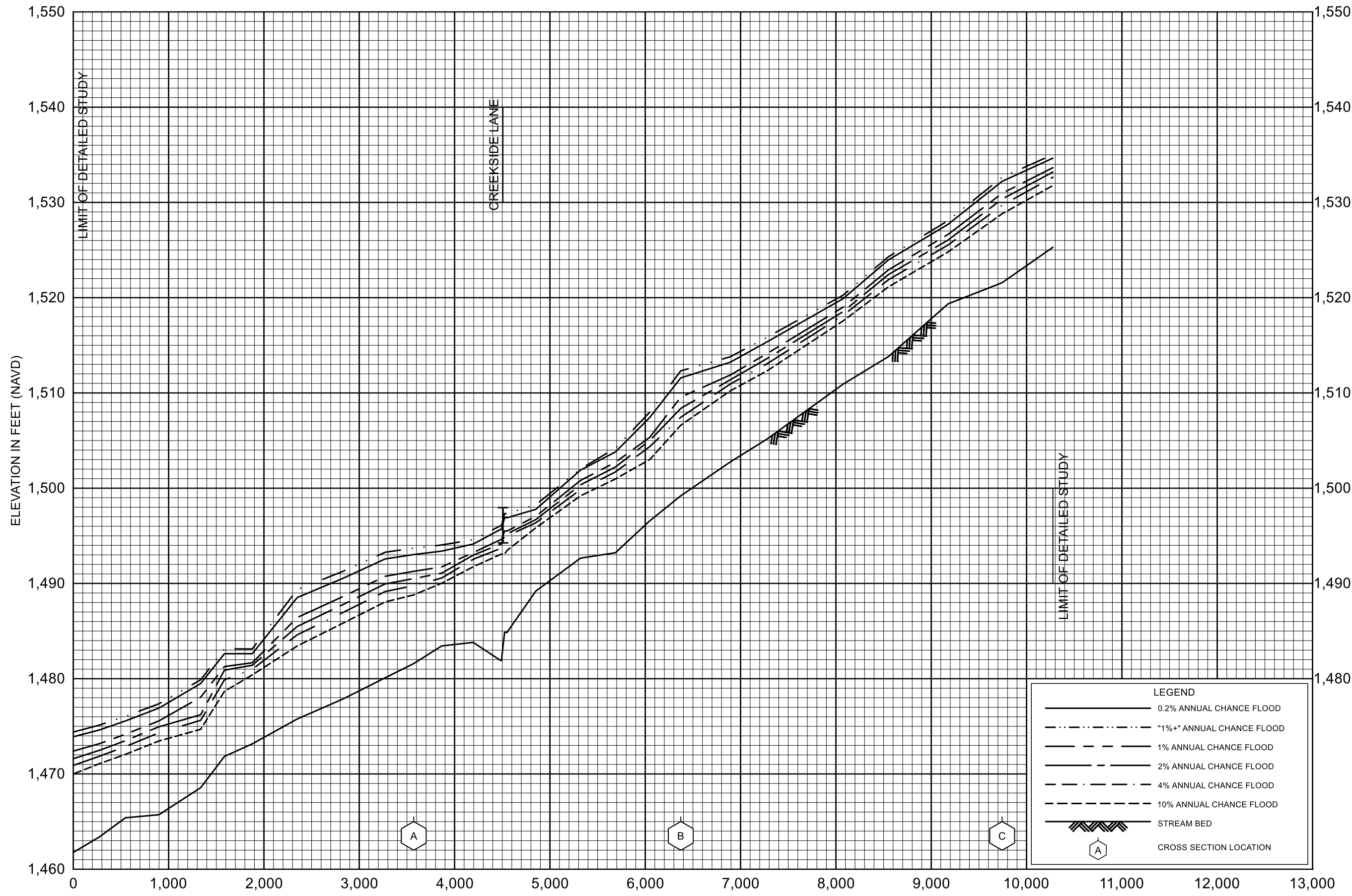
STREAM DISTANCE IN FEET ABOVE LIMIT OF DETAILED STUDY (LIMIT OF DETAILED STUDY IS APPROXIMATELY 20,006 FEET FROM CONFLUENCE WITH NEW RIVER)
