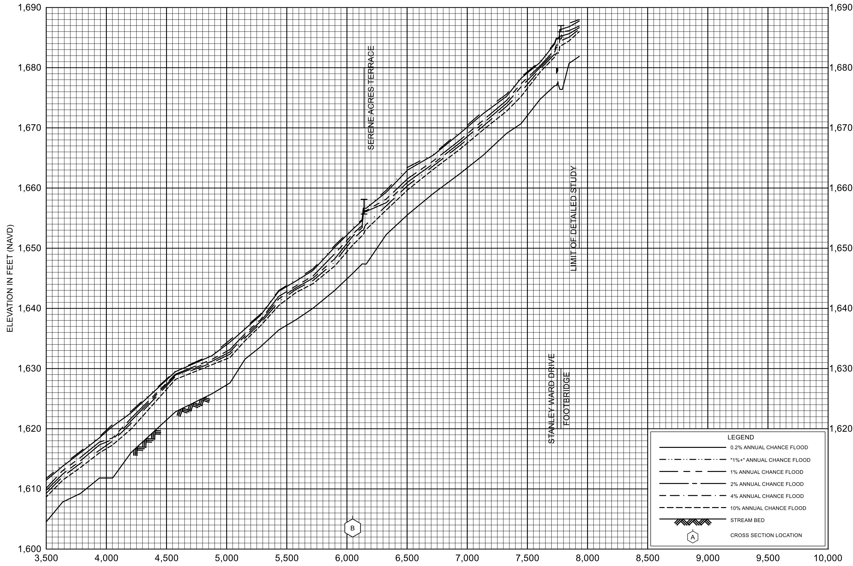
STREAM DISTANCE IN FEET ABOVE LIMIT OF DETAILED STUDY (LIMIT OF DETAILED STUDY IS APPROXIMATELY 7,717 FEET FROM CONFLUENCE WITH BLUESTONE RIVER)
