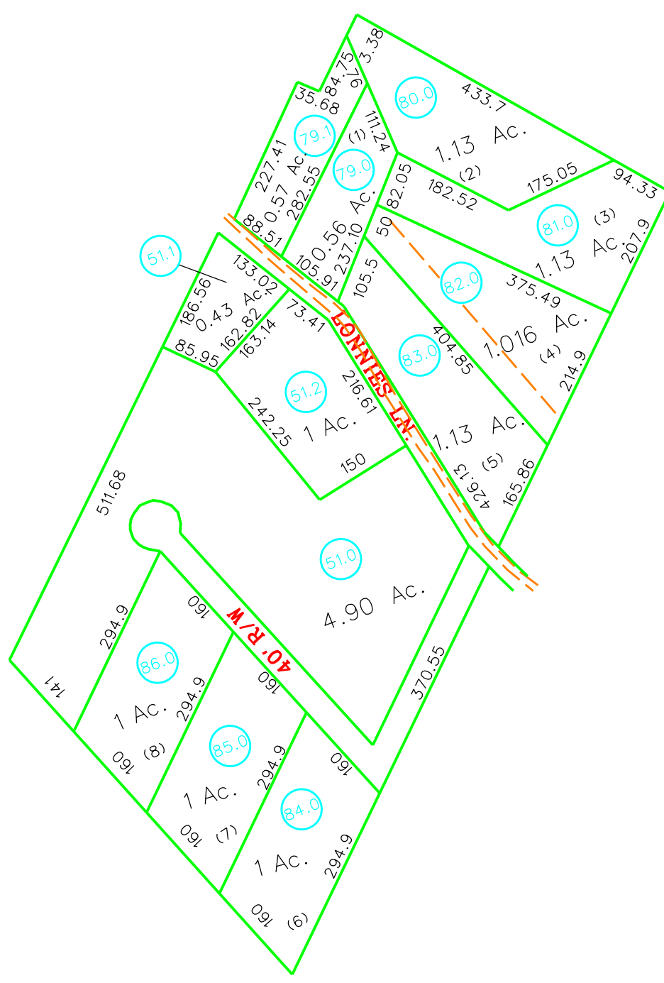
INSET NO.1 SCALE 1"=200'
