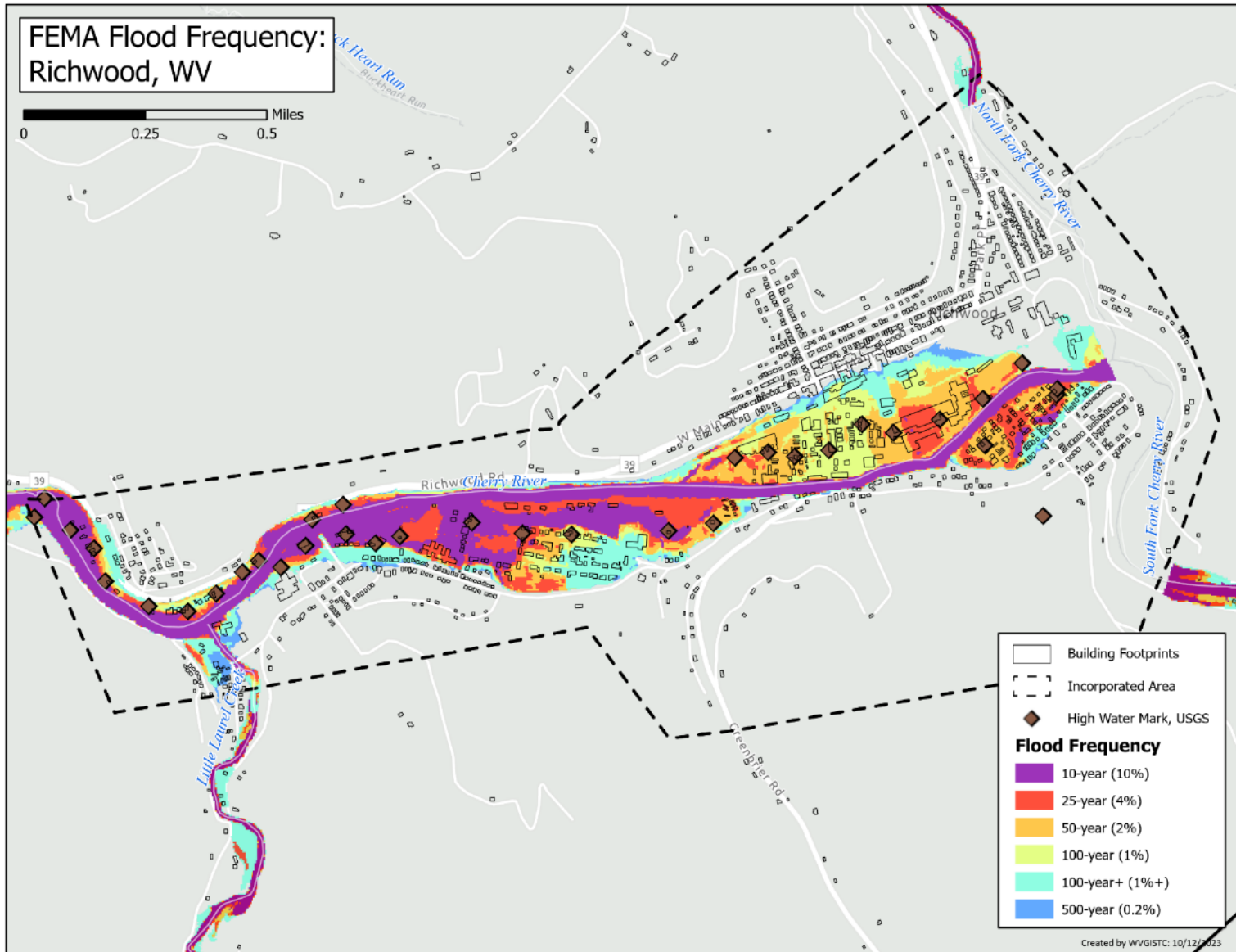
Figure 23. FEMA flood frequency map for Richwood
