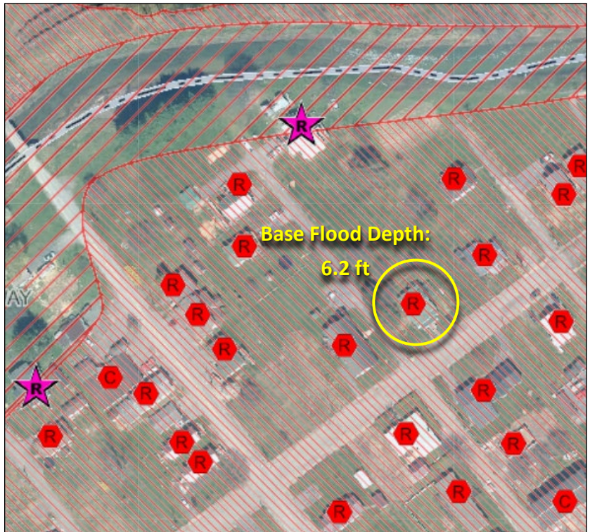
Figure 43. Structure with the maximum flood depth in Rainelle (Building ID: 13-13-0001-0085-0000 417 )
