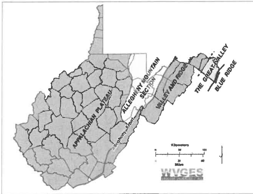
Figure 1. Different physiographic provinces of West Virginia (WVGES; http://www.wvgs.wvnet.edu/www/geology/geolphyp.htm )
