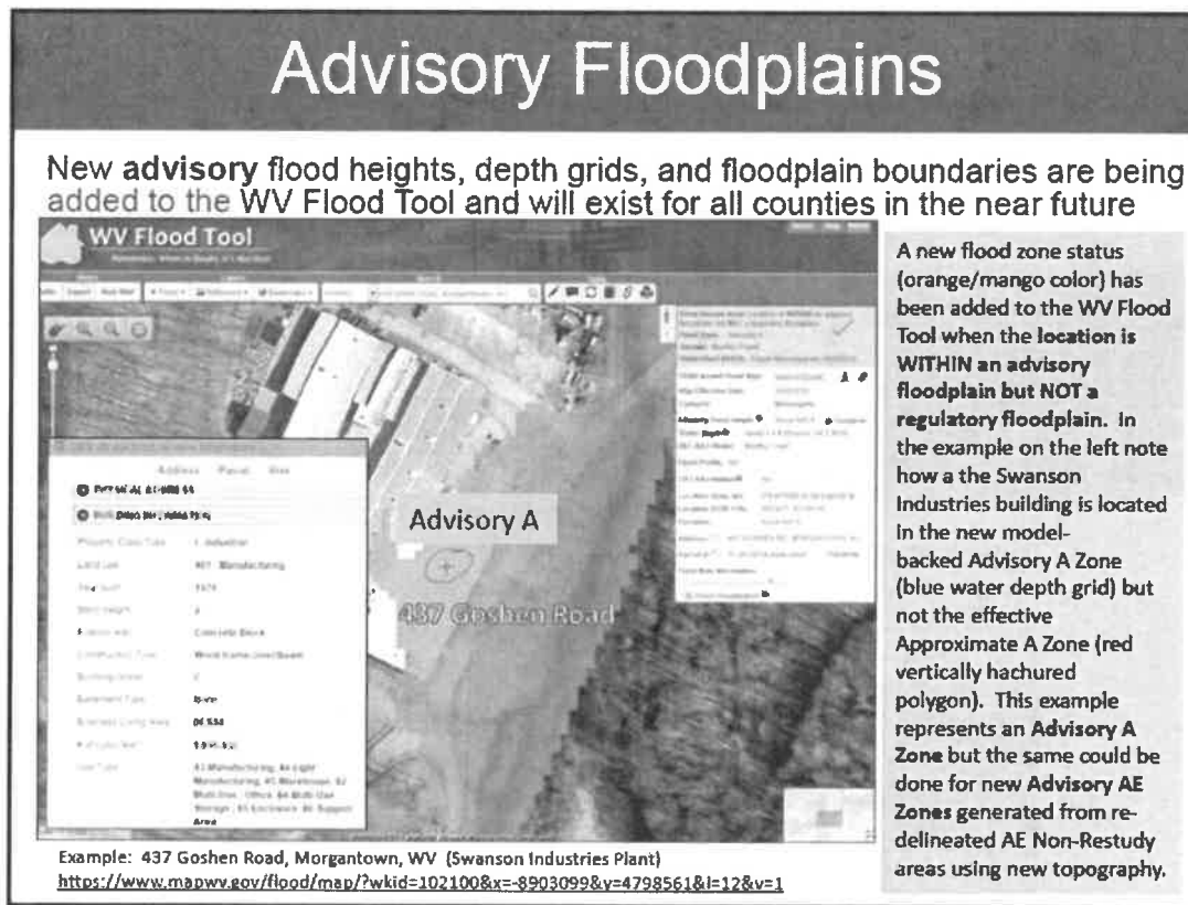
Figure 5. Model-backed Advisory A Zone flood heights and depth grids exist for 27 West Virginia counties, with the remainder 28 counties to be completed in several years.
