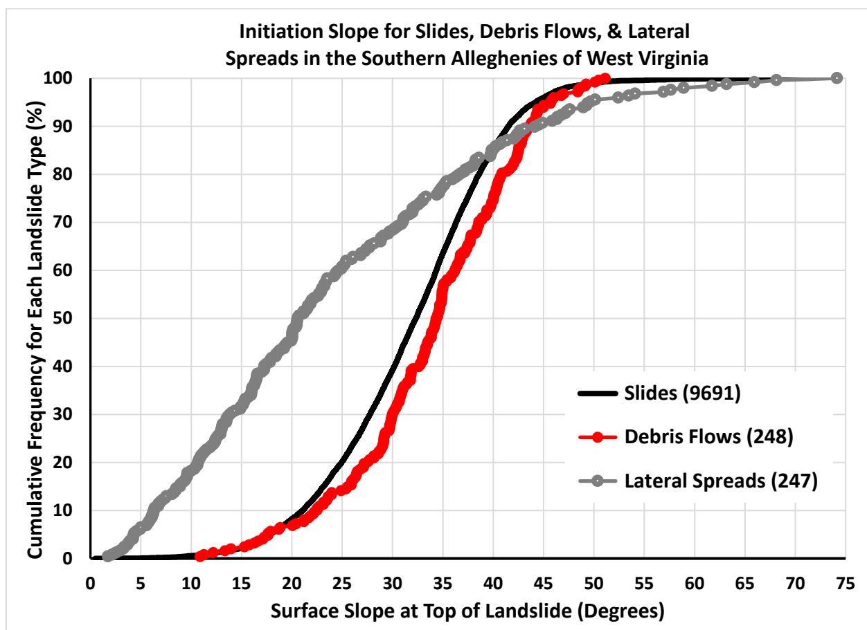
Figure 1. Comparison of initiation slopes for slides (including slumps), debris flows, and lateral spreads (rock cities) in the Southern Alleghenies of West Virginia. Initiation slope was measured at the uppermost point on a landslide as mapped from the LiDAR-based DEMs.
