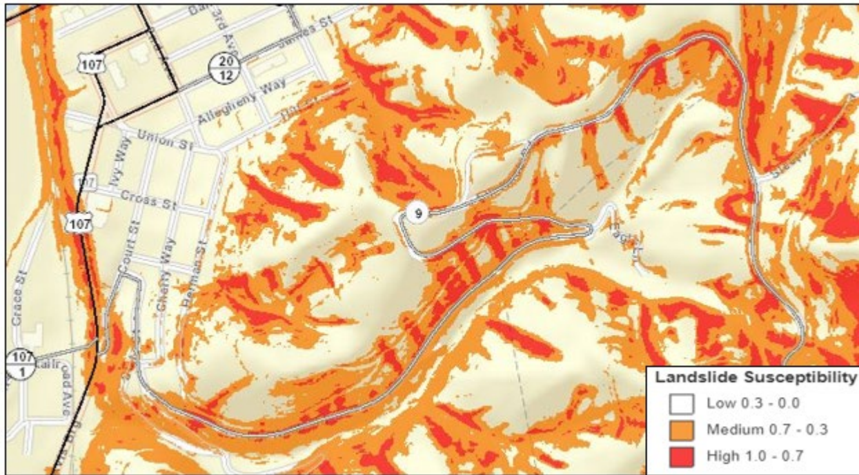
Landslide risk near Hinton, WV in Summers County
